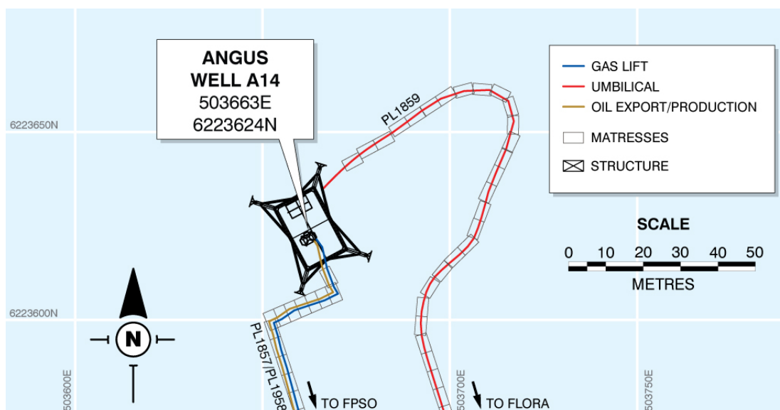
Figure F.2: Angus Well Centre and Infrastructure
