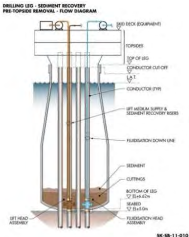
Figure 12-7: Flow Diagram of Sediment Recovery System with Topsides Removed
