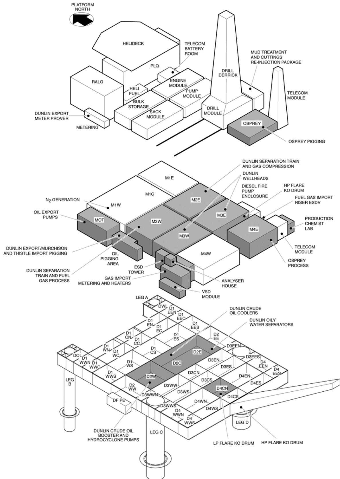
Figure 2-4: Dunlin Alpha Module Layout
