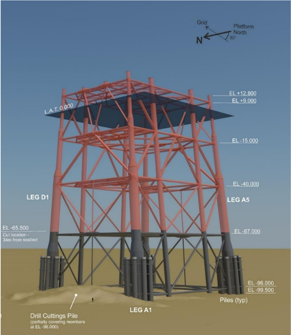
Figure 2.2: Complete Brae Bravo Jacket/Sub-structure
