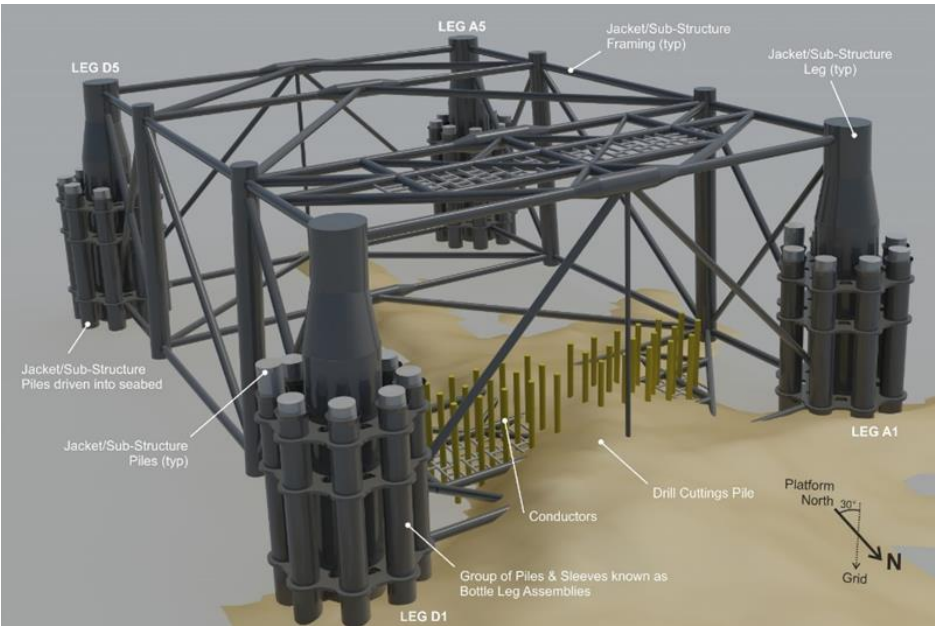
Figure 2.3: Brae Bravo Jacket/Sub-structure Footings
