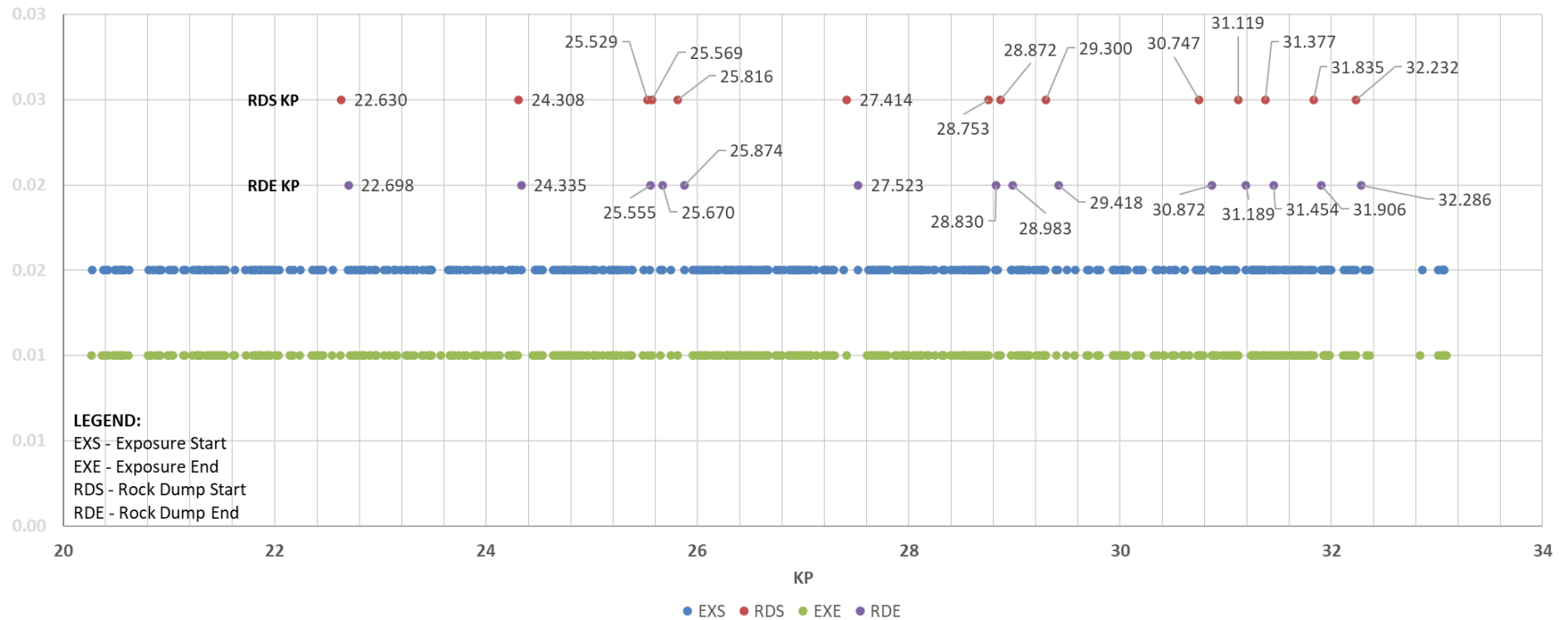
Figure B.1.1: PL9 rock vs. exposures plot KP20.0 to KP33.100 (2018 data)
