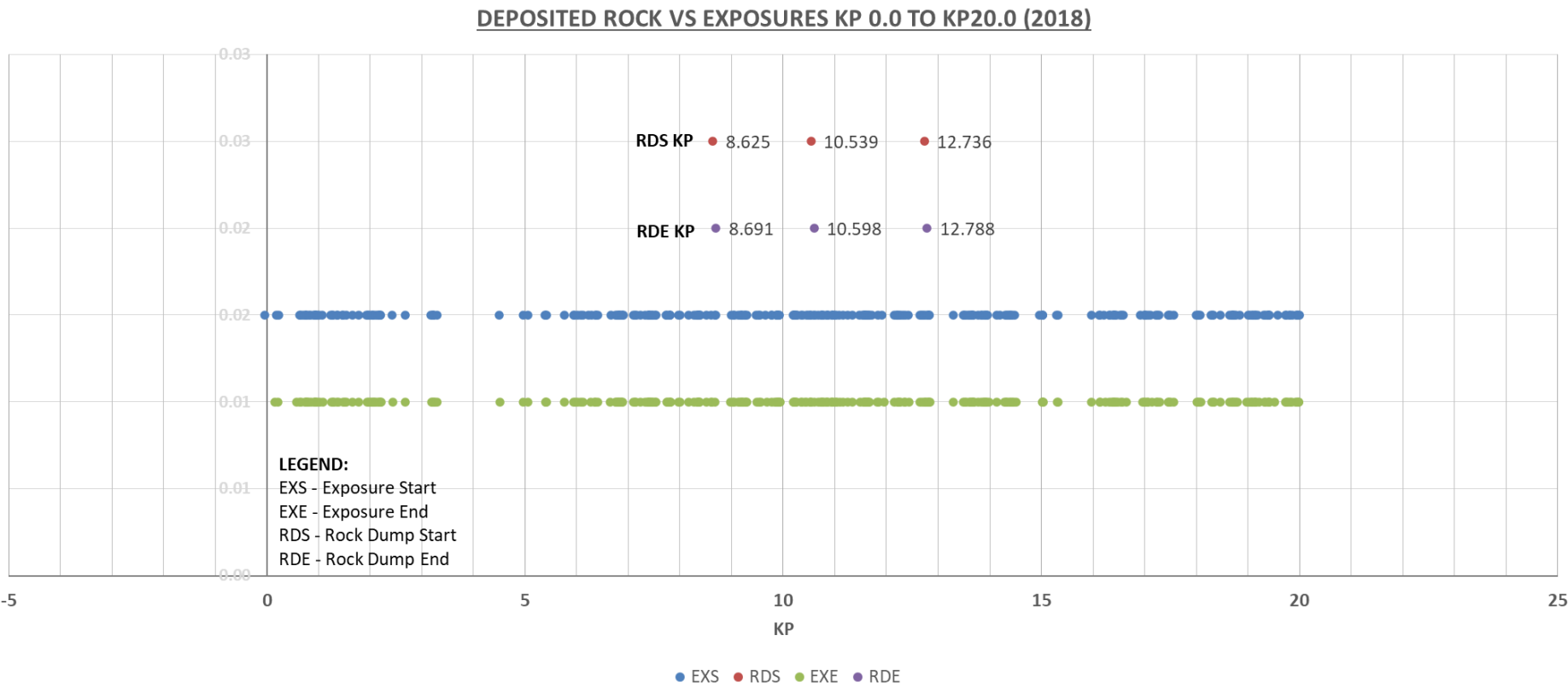
Figure B.1.1: PL9 rock vs. exposures plot KP0.0 to KP20.0 (2018 data)
