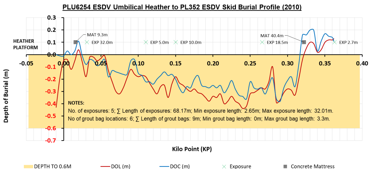
Figure 4.2.14: PLU6254 ESDV Umbilical burial profile (2010)
