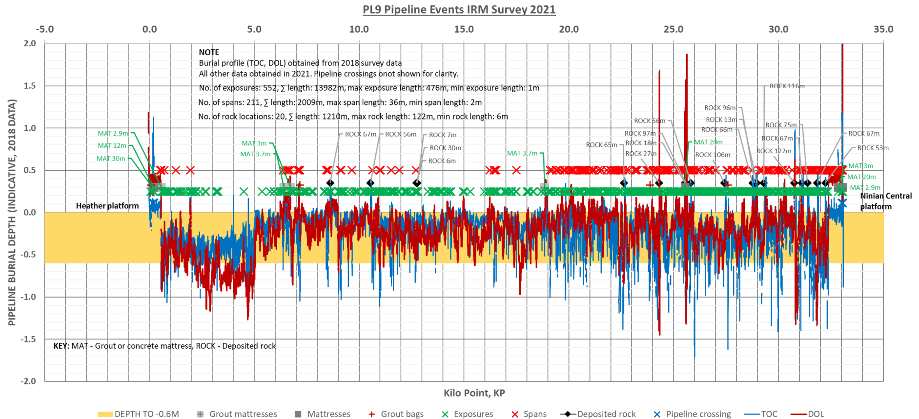
Figure 4.2.7: PL9 pipeline exposures, spans, mattresses, rock, etc. (2021) 5
