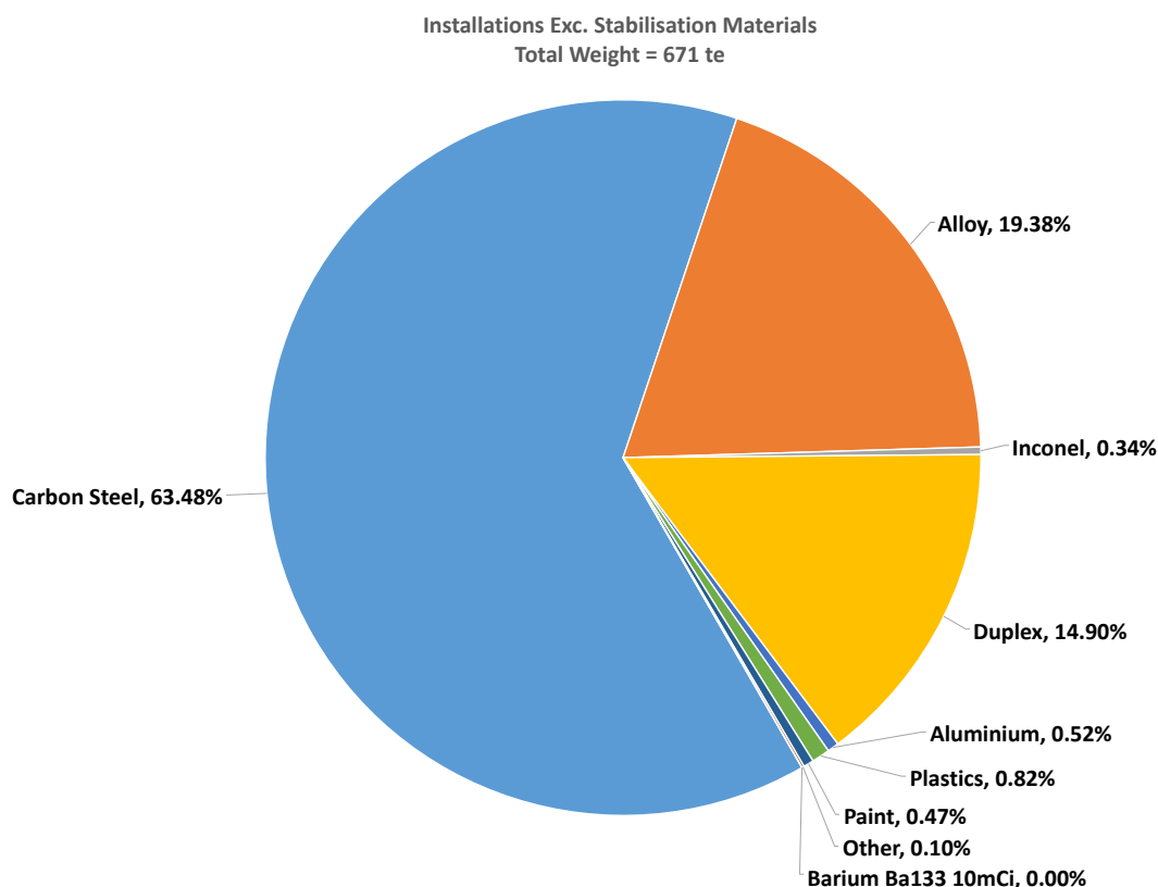
Figure 2-2 Subsea Installations Inventory – Excluding Stabilisation Material
