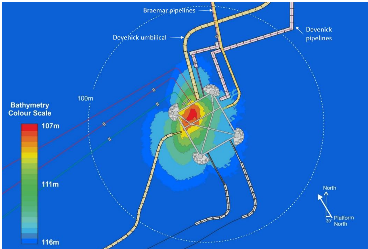
Figure 2-1 Location of the East Brae drill cuttings in relation to the subsea infrastructure.
