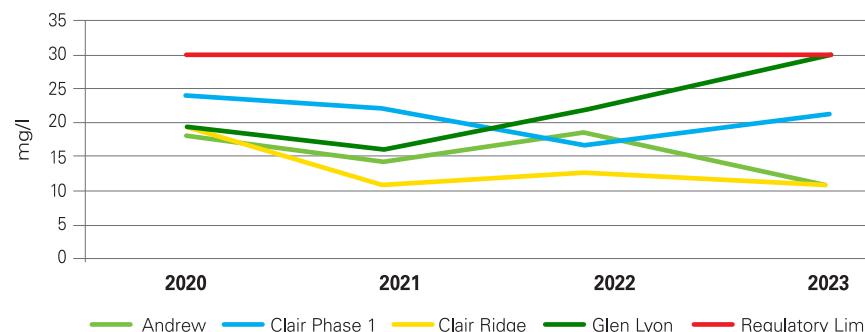
Figure 6: Annual average oil in produced water discharge between 2020 and 2023
