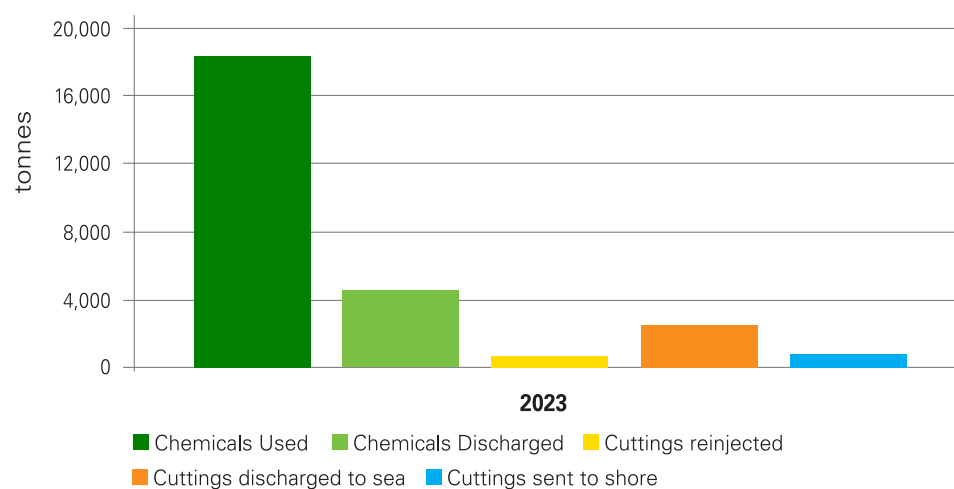
Figure 13: Drill cuttings (reinjected, discharged and disposed to landfill) and drilling chemicals used and discharged in 2023.
