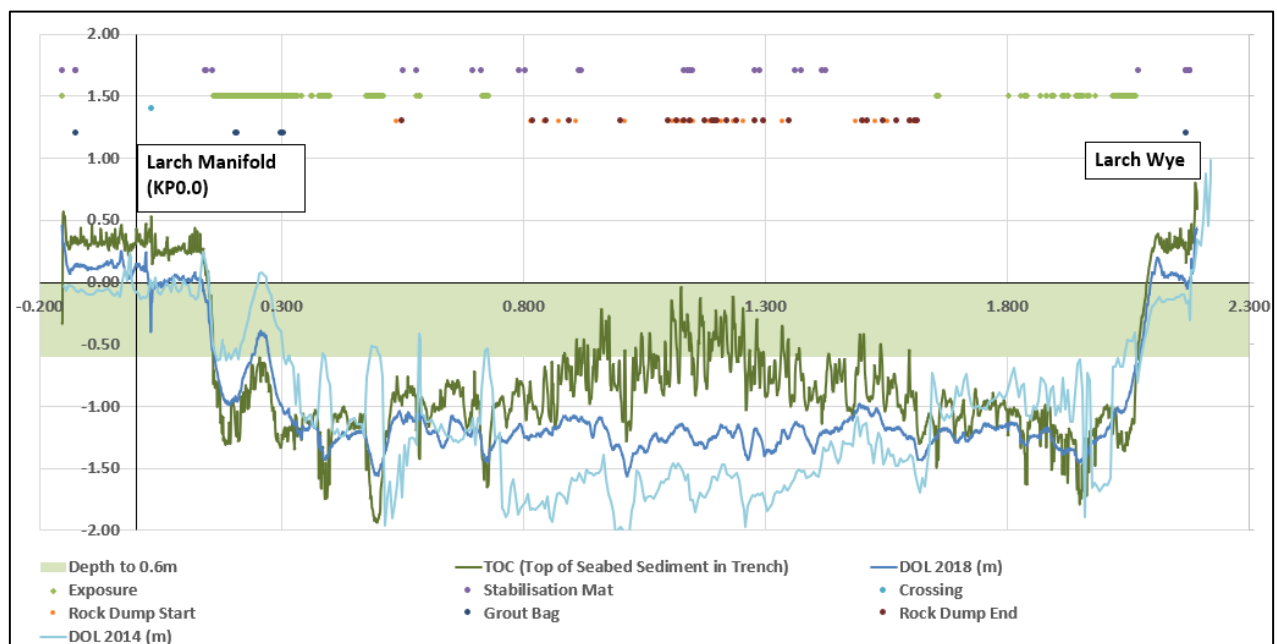
Figure 3-5: PL1527 10" Production Pipeline Burial Profile (2014 & 2018)
