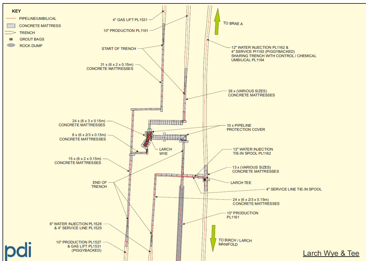
Figure A-3: Larch Wye Approaches
