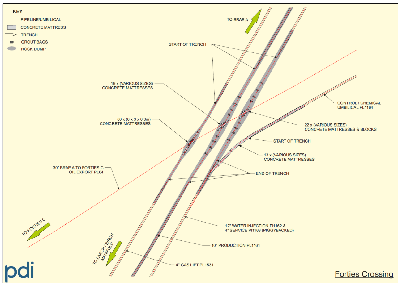
Figure A-2: Forties Crossing
