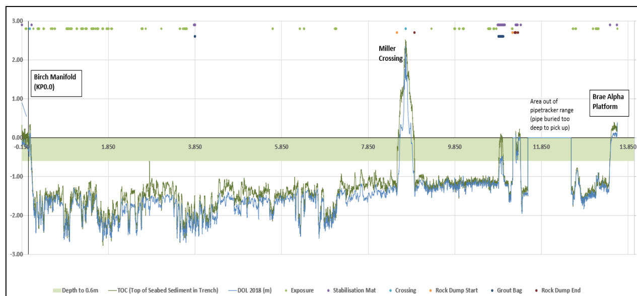
Figure 3-4: PL1164 Control / Chemical Umbilical Burial Profile (2018)
