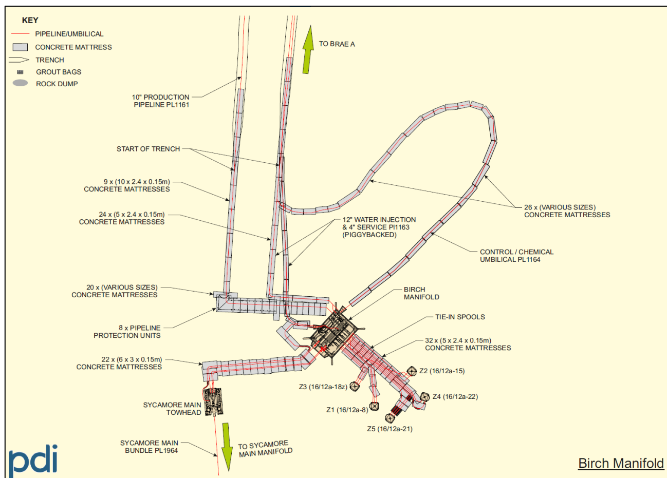
Figure A-5: Birch Manifold and Wells
