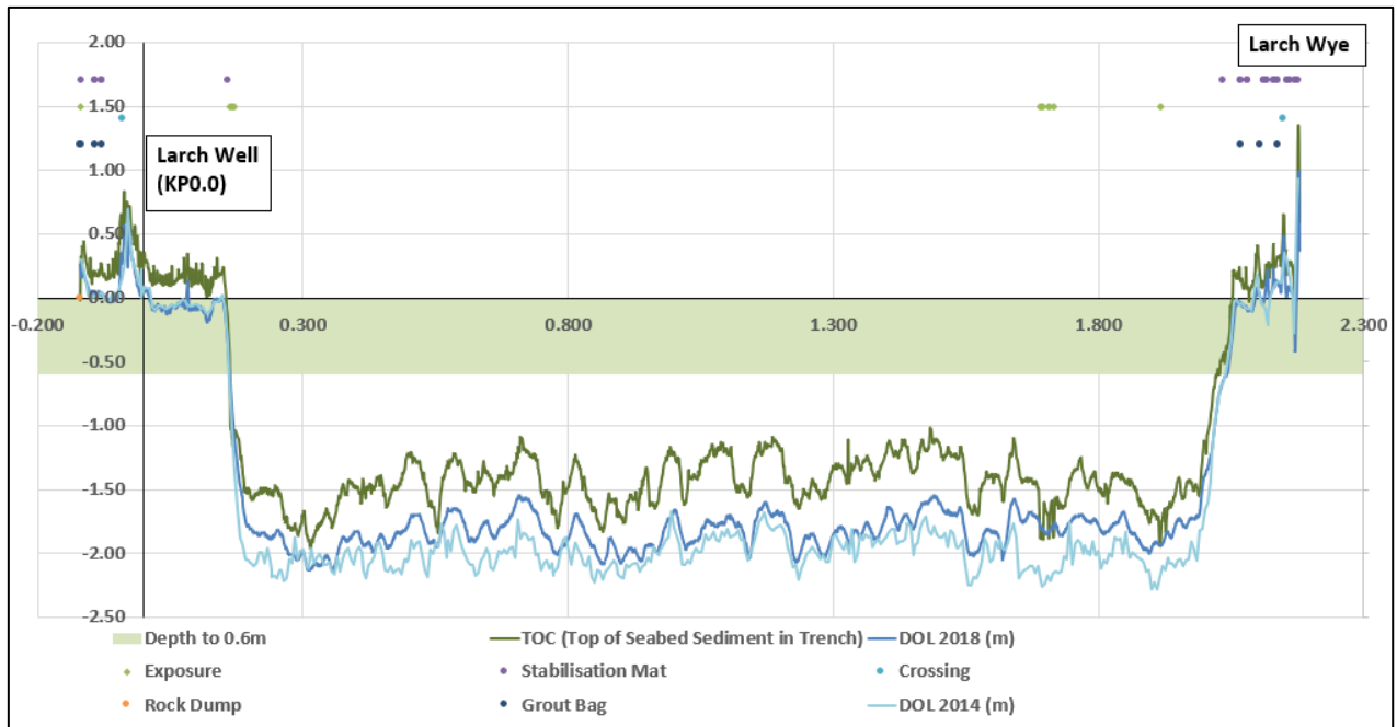
Figure 3-7: PL1528 6" WI Pipeline c/w Piggybacked PL1529 4" Service Pipeline Burial Profile (2014 & 2018)
