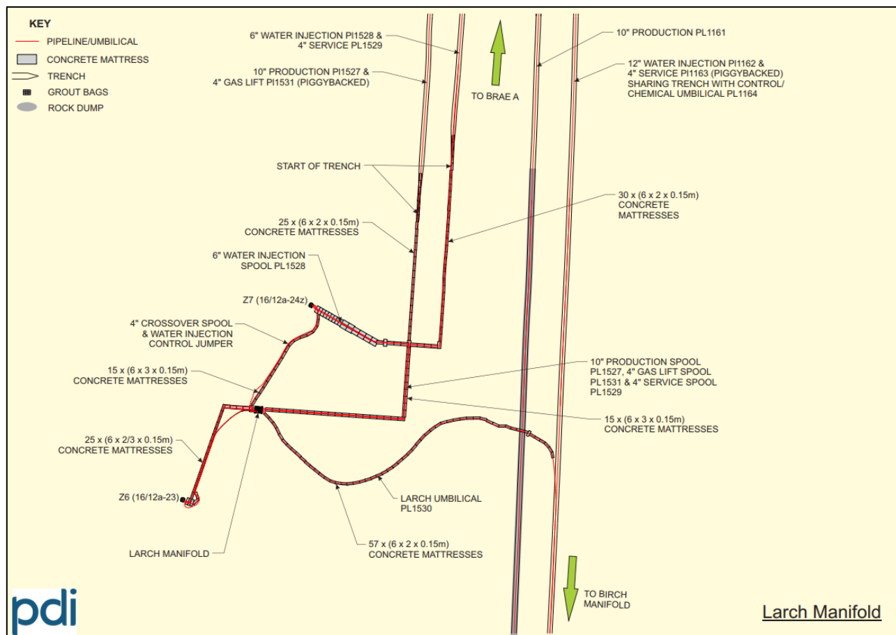
Figure A-4: Larch Gas Lift (& Production) Manifold & Wells
