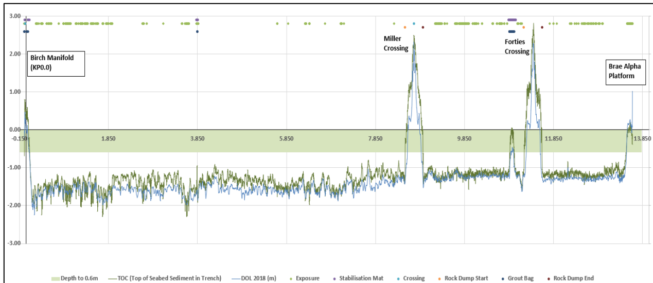
Figure 3-2: PL1162 12" WI Pipeline c/w Piggybacked PL1163 4" GL Pipeline Burial Profile (2018)
