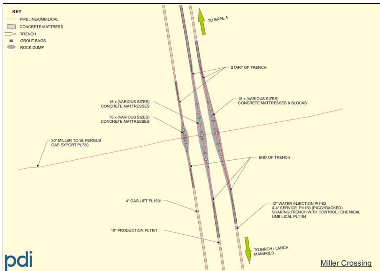
Figure A-1: Miller Crossing
