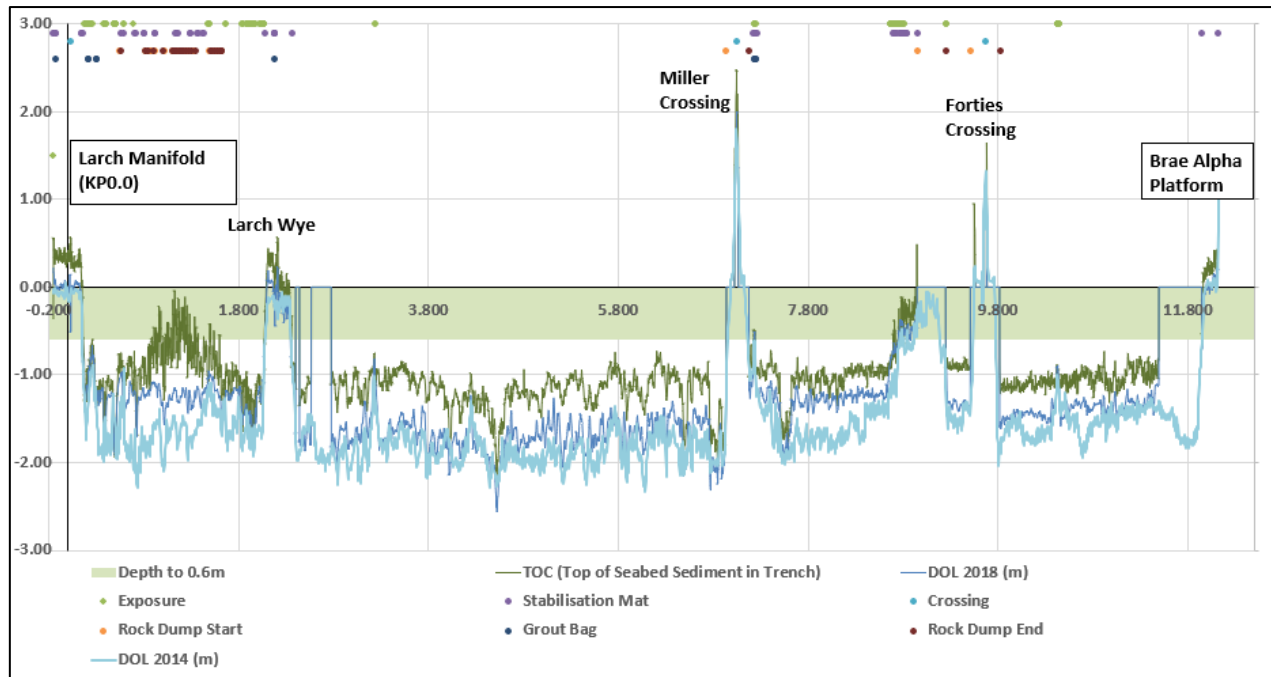
Figure 3-6: PL1531 4" GL Pipeline Burial Profile (2014 & 2018)
