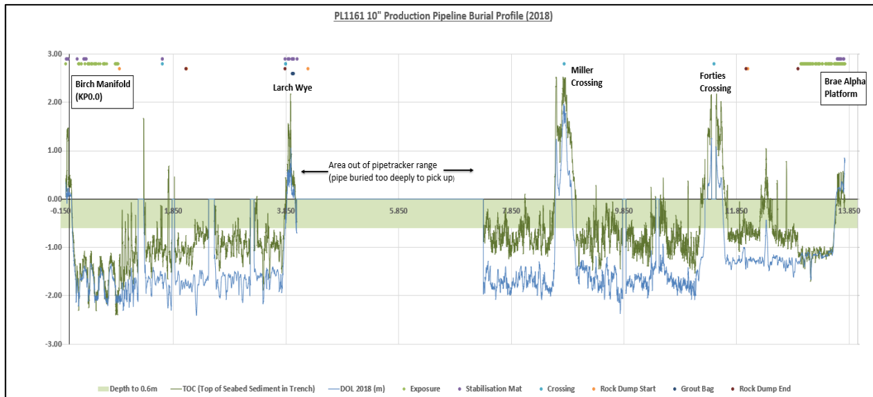
Figure 3-1: PL1161 10" Production Pipeline Burial Profile (2018)
